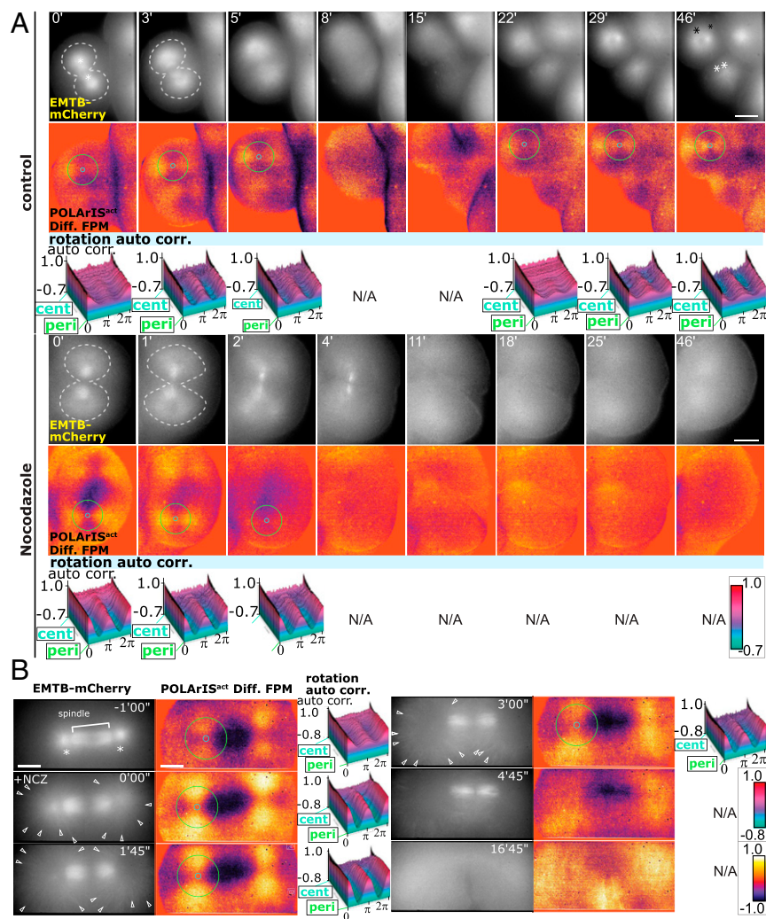
Fig. 6. FLARE dynamics is disrupted by inhibiting polymerization of microtubules. (A and B) Time-lapse two-axis FPM observation of dimethyl sulfoxide (control) or nocodazole-treated embryos expressing POLArIS act and EMTB-mCherry in the fourth (A) and the third cleavages (B). (A) Top rows show vertical polarization images of EMTB-mCherry (asterisks indicate centrosomes, dashed lines indicate contours of microtubule asters), middle rows show differential FPM images of POLArIS act with circles of min/max diameters used in autocorrelation analyses, and bottom rows show 3D plots of autocorrelation analyses of FLARE. N/A means that no center of the cross pattern was identified in our search algorithm. The drug was added at time 0. (Scale bar: 50 \mu\text{m} .) (B) Left columns show vertical polarization images of EMTB-mCherry (asterisks indicate centrosomes), middle columns show differential FPM images with circles of min/max diameters used in autocorrelation analyses, and right columns show 3D plots of autocorrelation analyses of FLARE structures. N/A means that no center of the cross pattern was identified in our search algorithm. The drug was added after at least one astral microtubule reached the cell surface (time 0). A silicone immersion 40 \times objective lens and a 1.5 \times intermediate magnification lens were used to visualize microtubule filaments (arrowheads). (Scale bar: 25 \mu\text{m} .)
